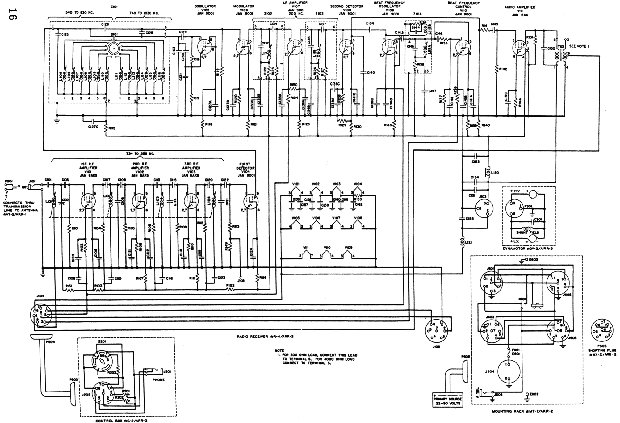
SCHEMATIC DIAGRAM RADIO RECEIVER ARR-2
