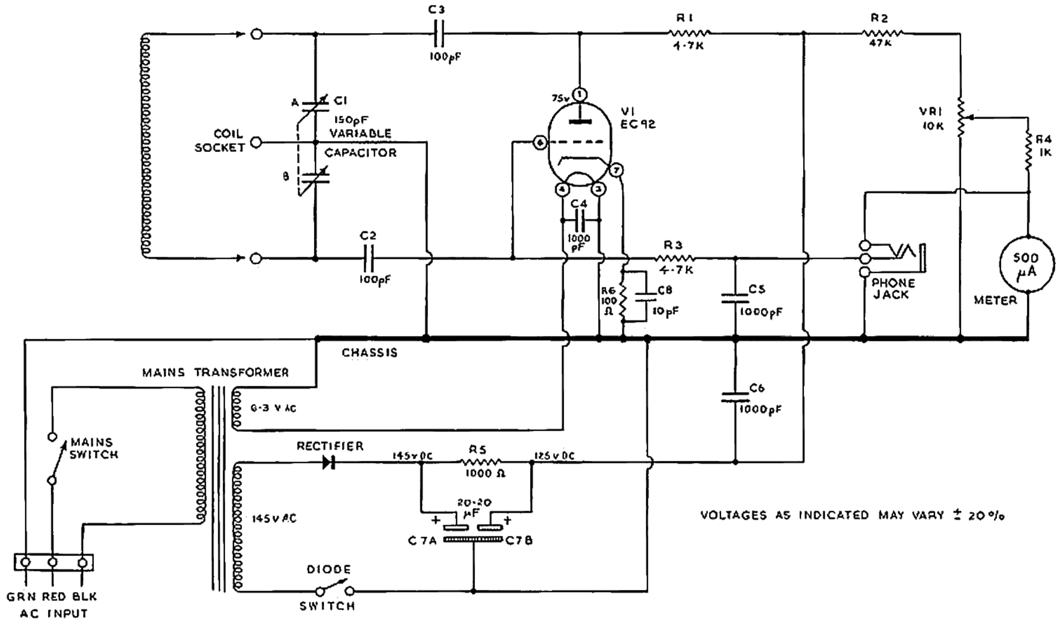
HEATHKIT GRID DIP METER MODEL GD-1U CIRCUIT DIAGRAM
