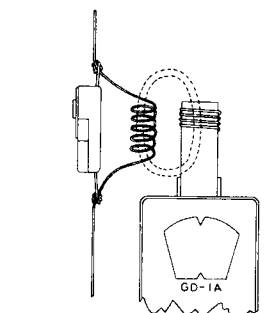
Inductive coupling to a coil.
