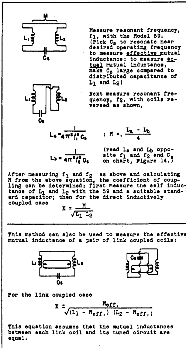
Figure 15 MEASUREMENT OF MUTUAL INDUCTANCE
