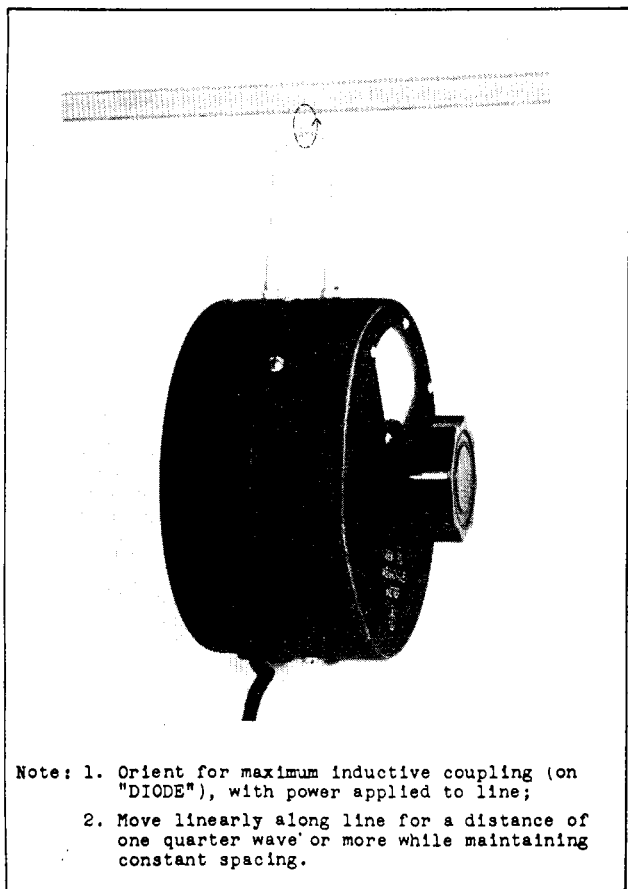
Figure 10 - CHECKING FOR STANDING WAVES ON TRANSMISSION LINES
