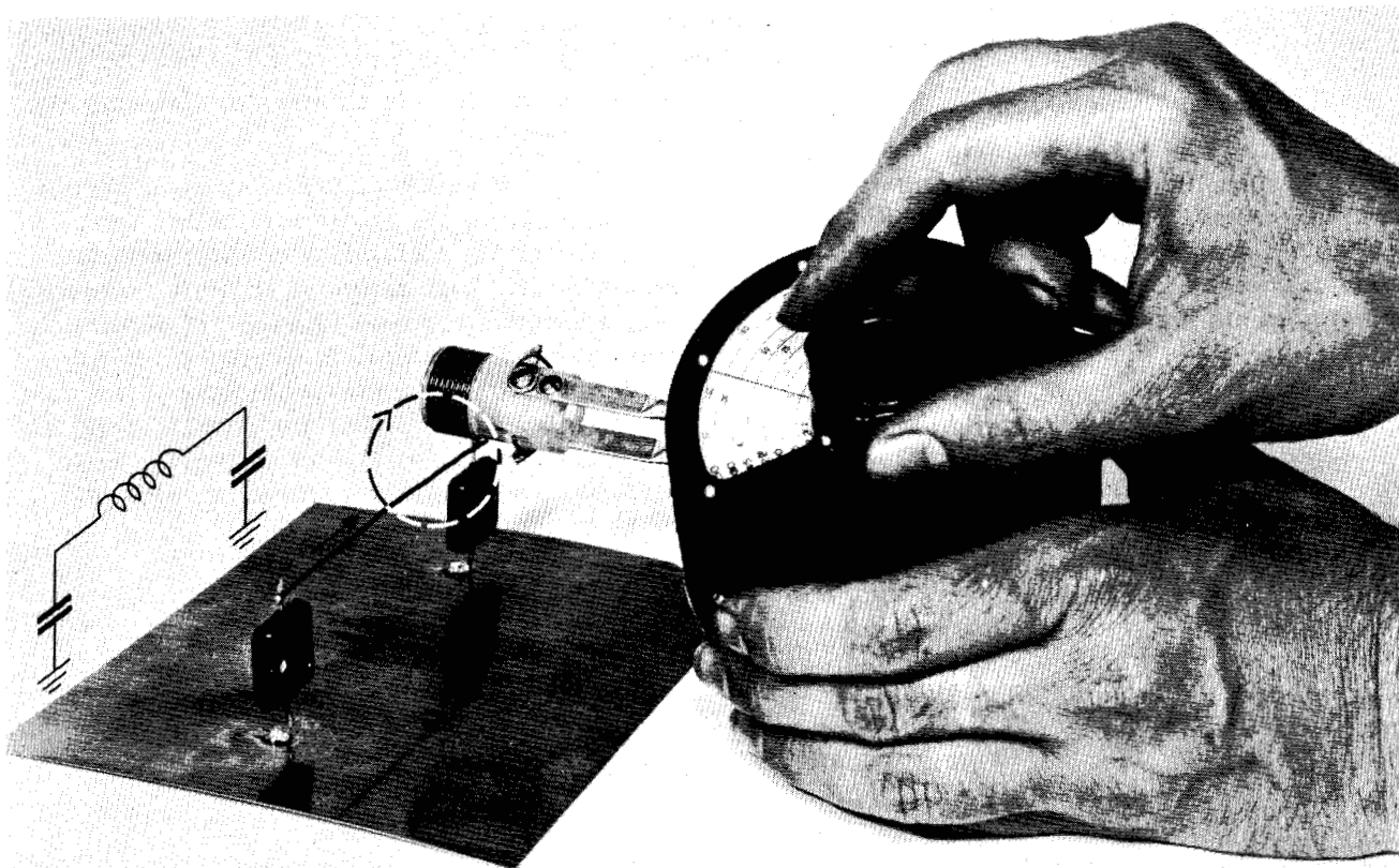
Figure 2 - USE OF INDUCTIVE COUPLING
