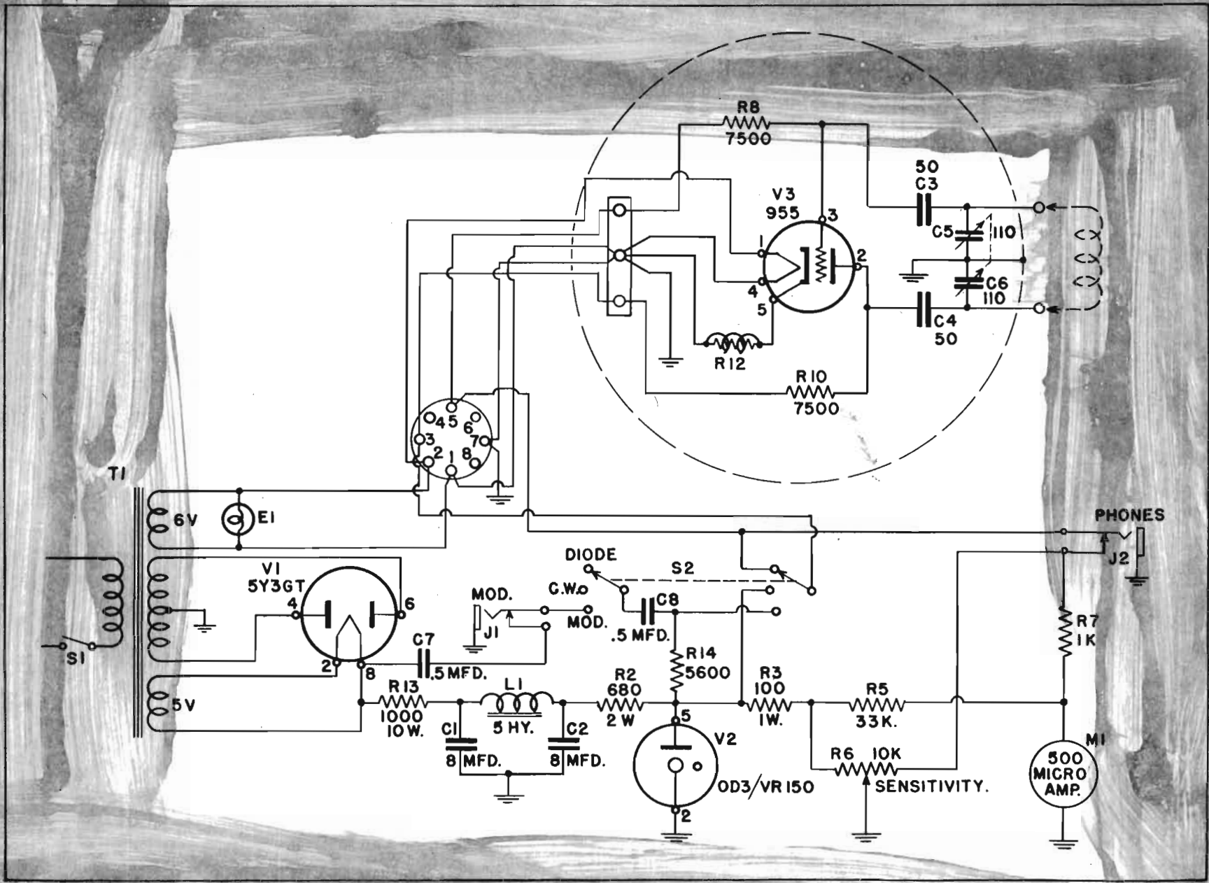
Figure 18 - SCHEMATIC DIAGRAM
