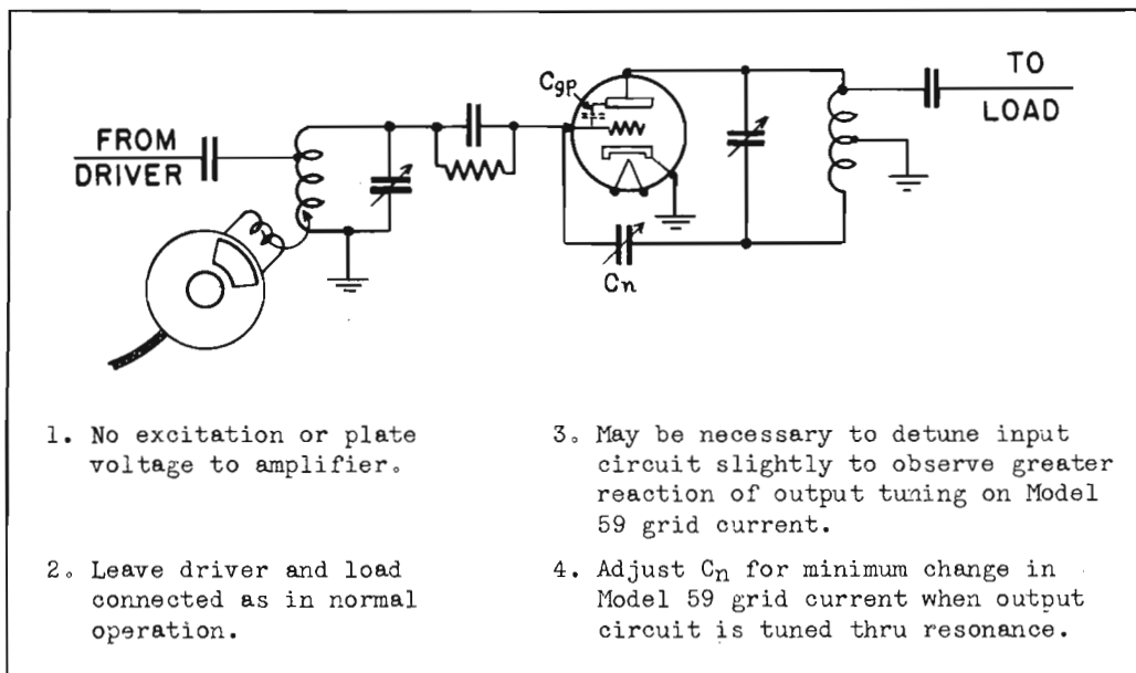
Figure 8 - REACTION METHOD OF NEUTRALIZATION (Model 59 in "CW" Position)
