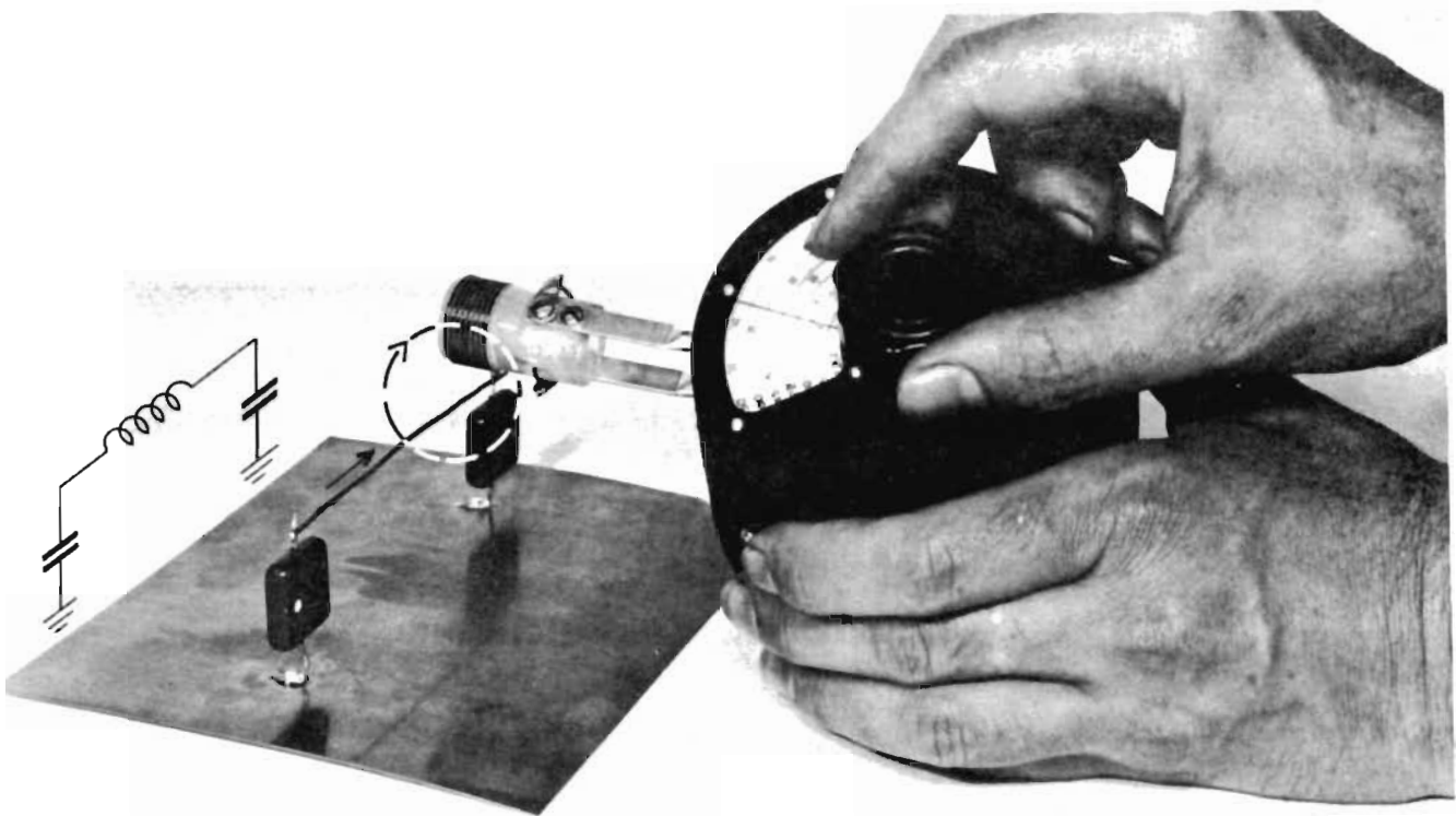
Figure 2 - USE OF INDUCTIVE COUPLING
