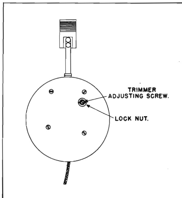
Figure 17 - ADJUSTMENT OF TRIMMER
