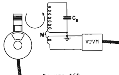
Figure 16C REDUCTION OF VTVM LOADING BY INDUCTIVE COUPLING
