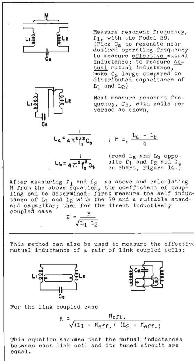
Figure 15 MEASUREMENT OF MUTUAL INDUCTANCE
