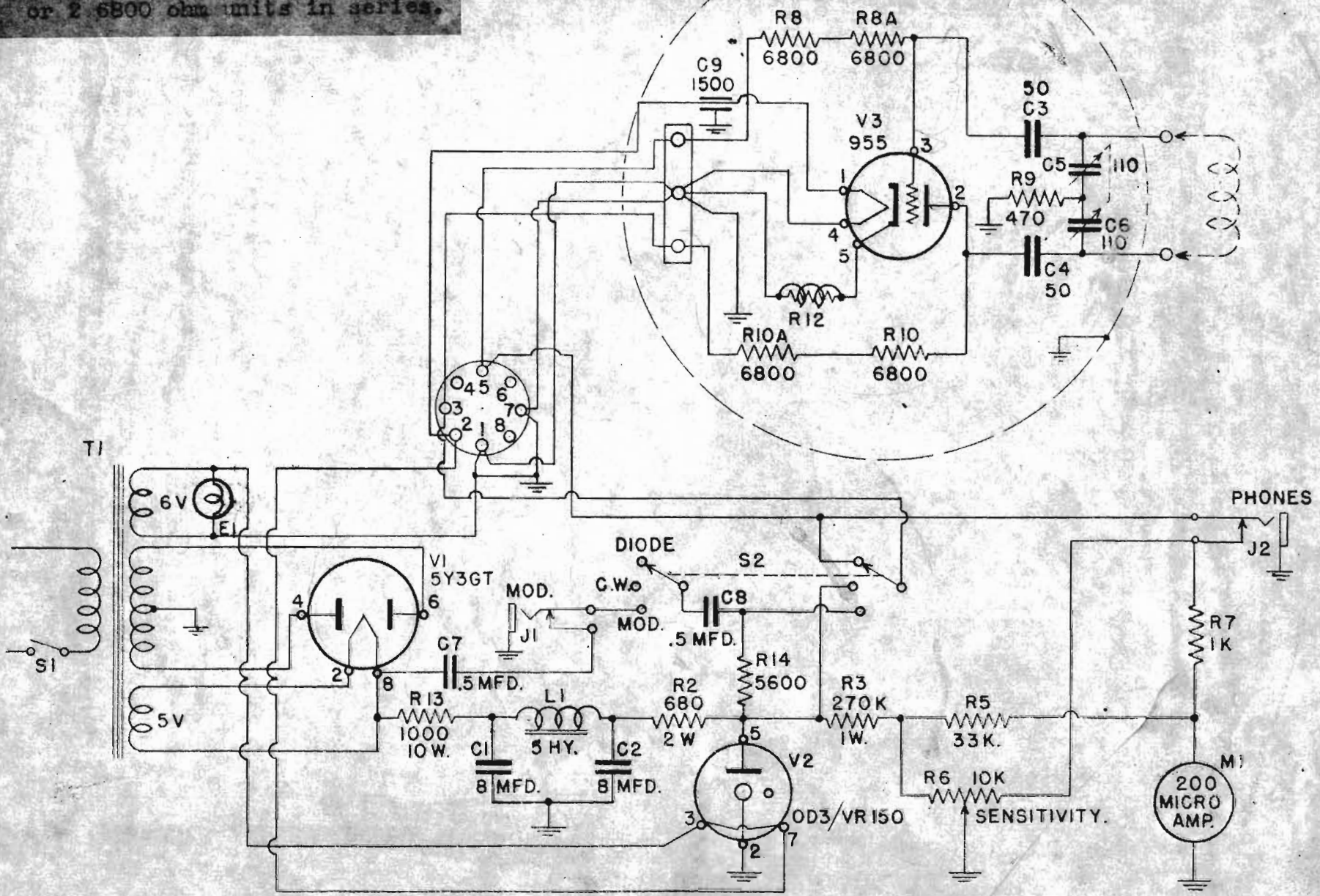
FIG.18 - SCHEMATIC DIAGRAM.
